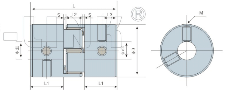
LK20-40~LK20-105
